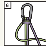
6 Next, take the right side cords over the top of the crossed left
